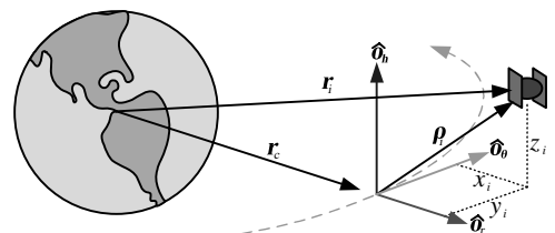
Fig. 1 Illustration of rotating Hill coordinate frame.
